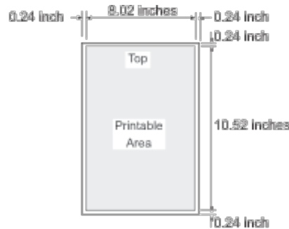
Figure 26. Recommended Printable Area for an 8.5 x 11-Inch Sheet on the Infoprint 2105 Printer
