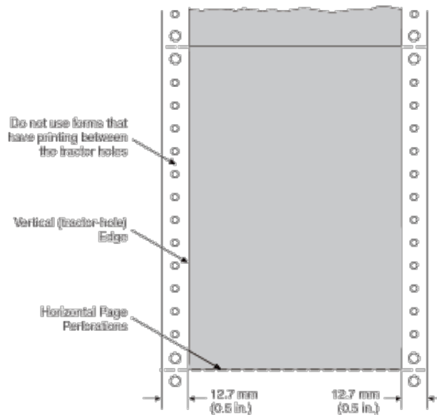
Figure 38. Printable Area on the Infoprint 4000-ID1/ID2 and 4000-ID3/ID4 Printers
